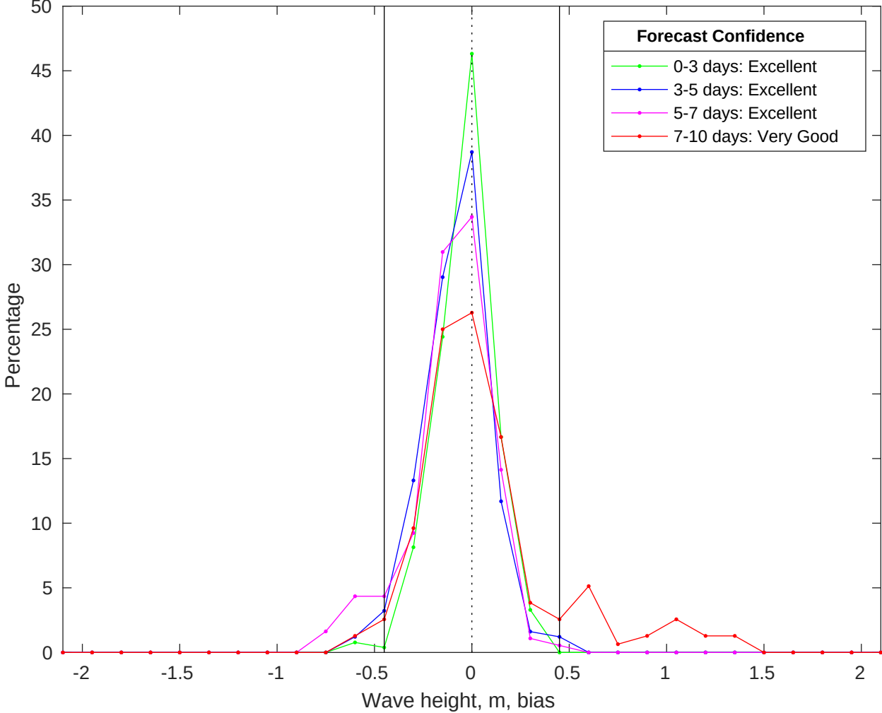
NDBC 51000 vs CMEMS Waves Bias Histogram: 23-Oct-2025
