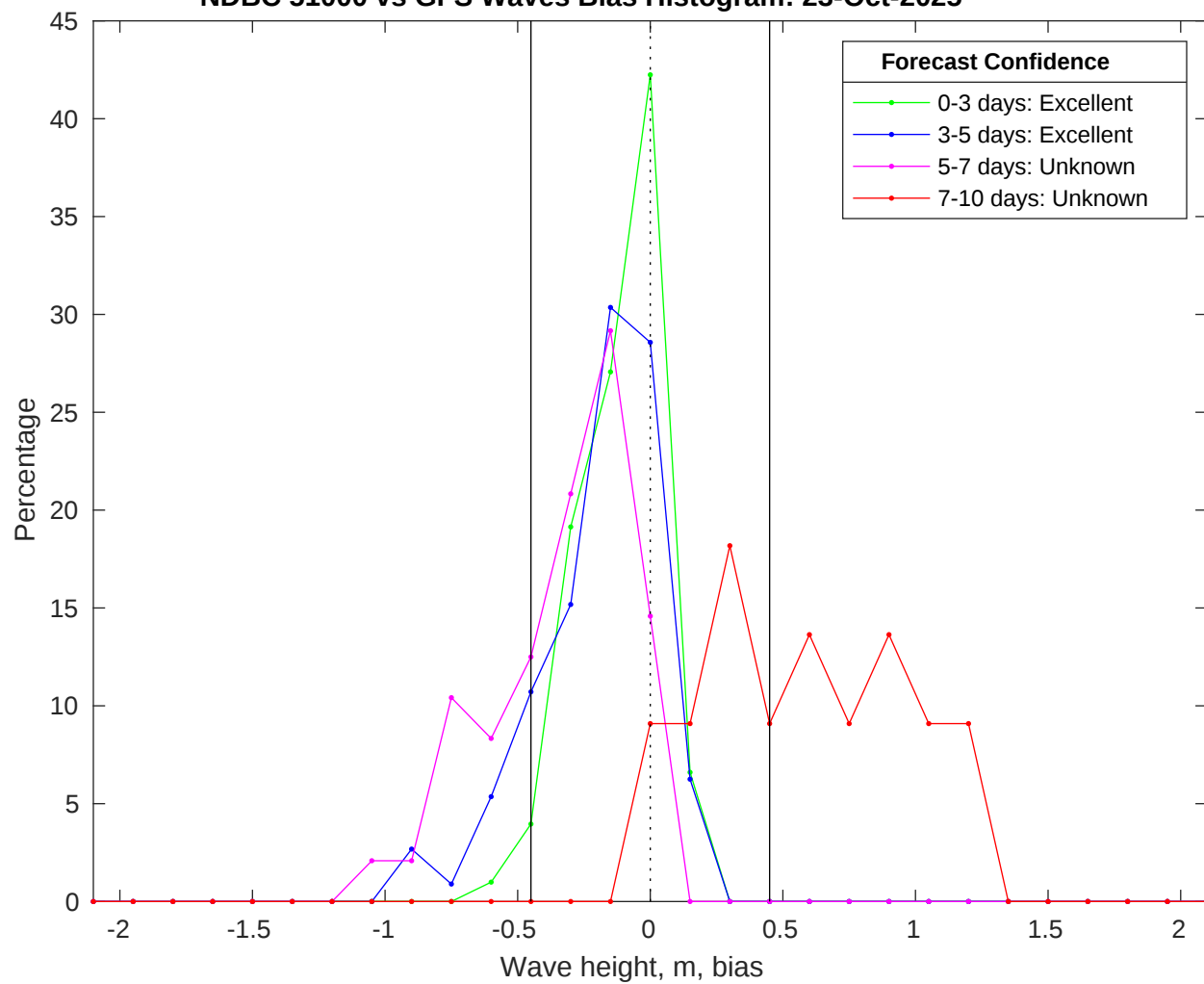
NDBC 51000 vs GFS Waves Bias Histogram: 23-Oct-2025
