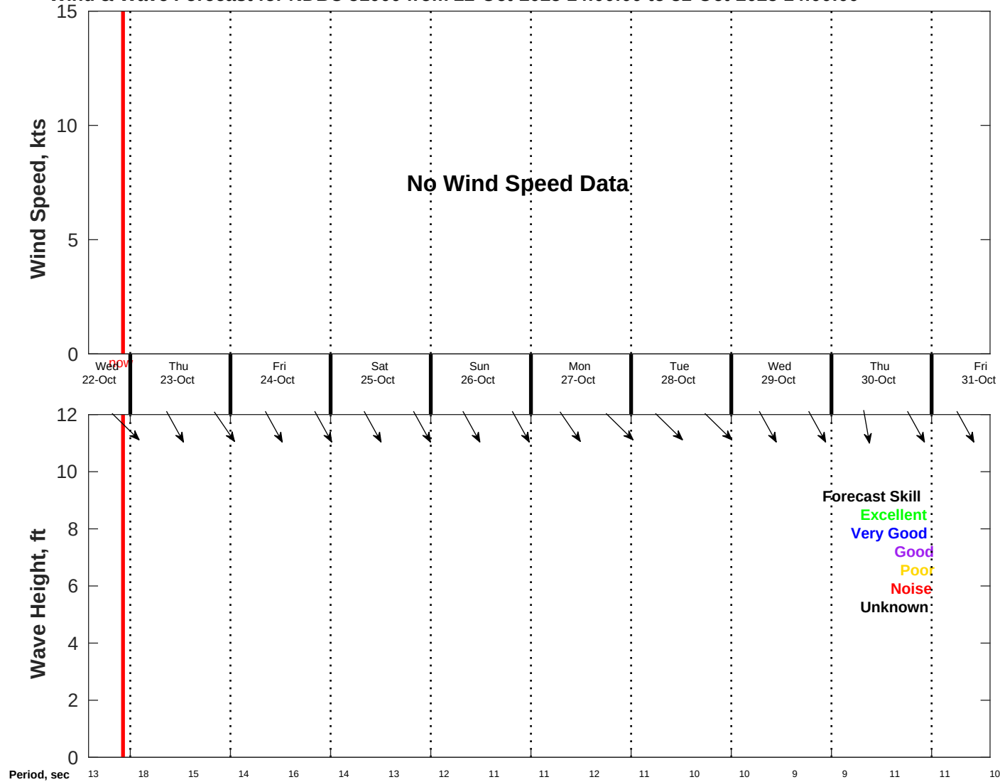
Wind & Wave Forecast for NDBC 51000 from 22-Oct-2025 14:00:00 to 31-Oct-2025 14:00:00
