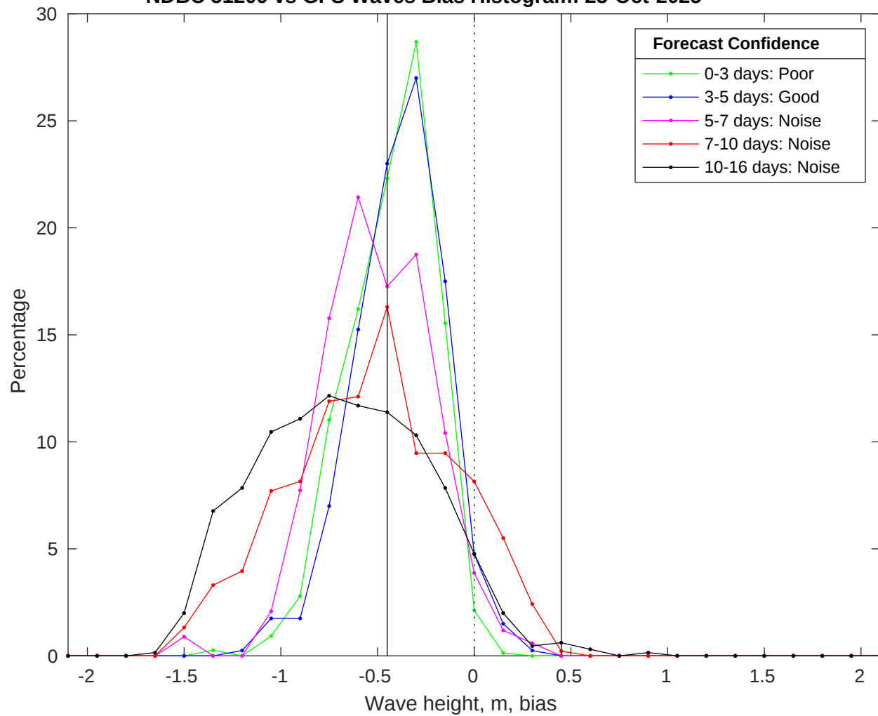
NDBC 51209 vs GFS Waves Bias Histogram: 23-Oct-2025
