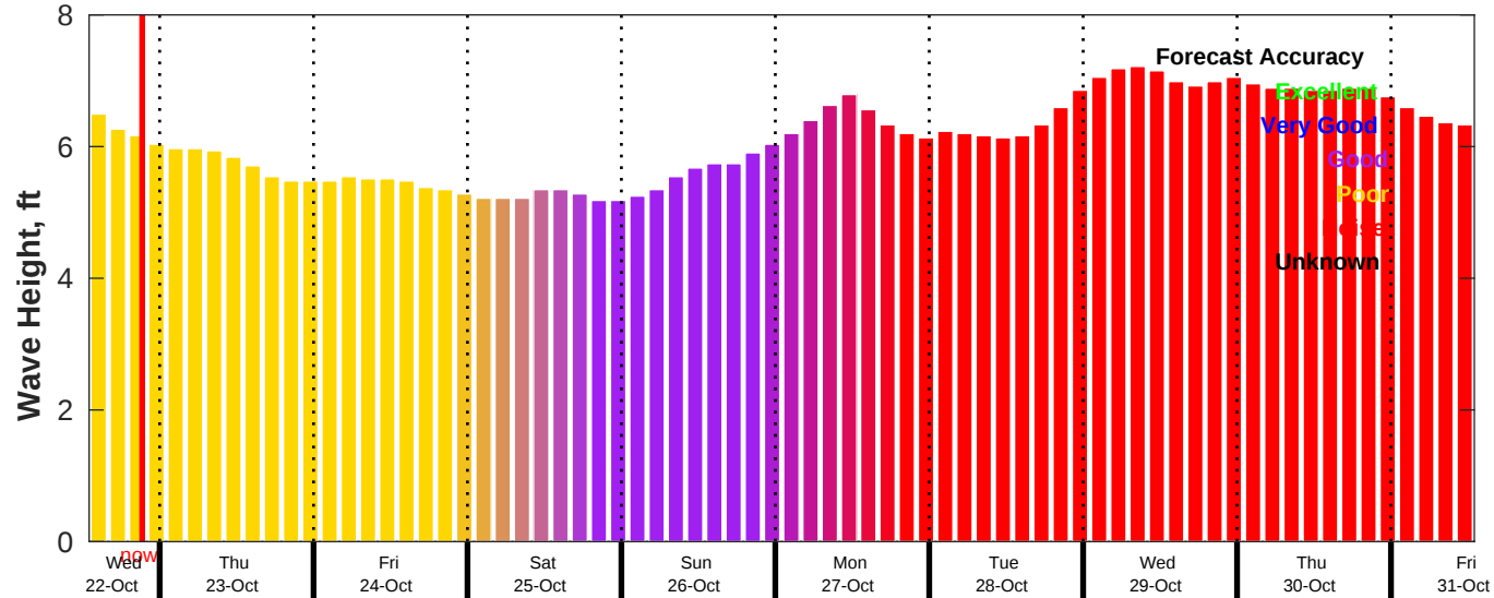
GFS Wave Forecast for NDBC 51209 from 22-Oct-2025 13:00:00 to 31-Oct-2025 13:00:00
