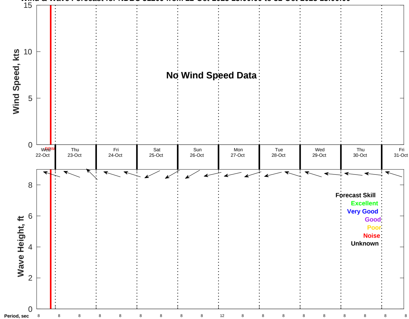
Wind & Wave Forecast for NDBC 51209 from 22-Oct-2025 13:00:00 to 31-Oct-2025 13:00:00
