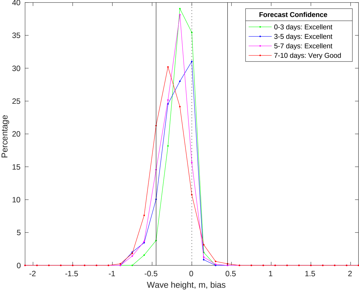
NDBC 52213 vs CMEMS Waves Bias Histogram: 23-Oct-2025
