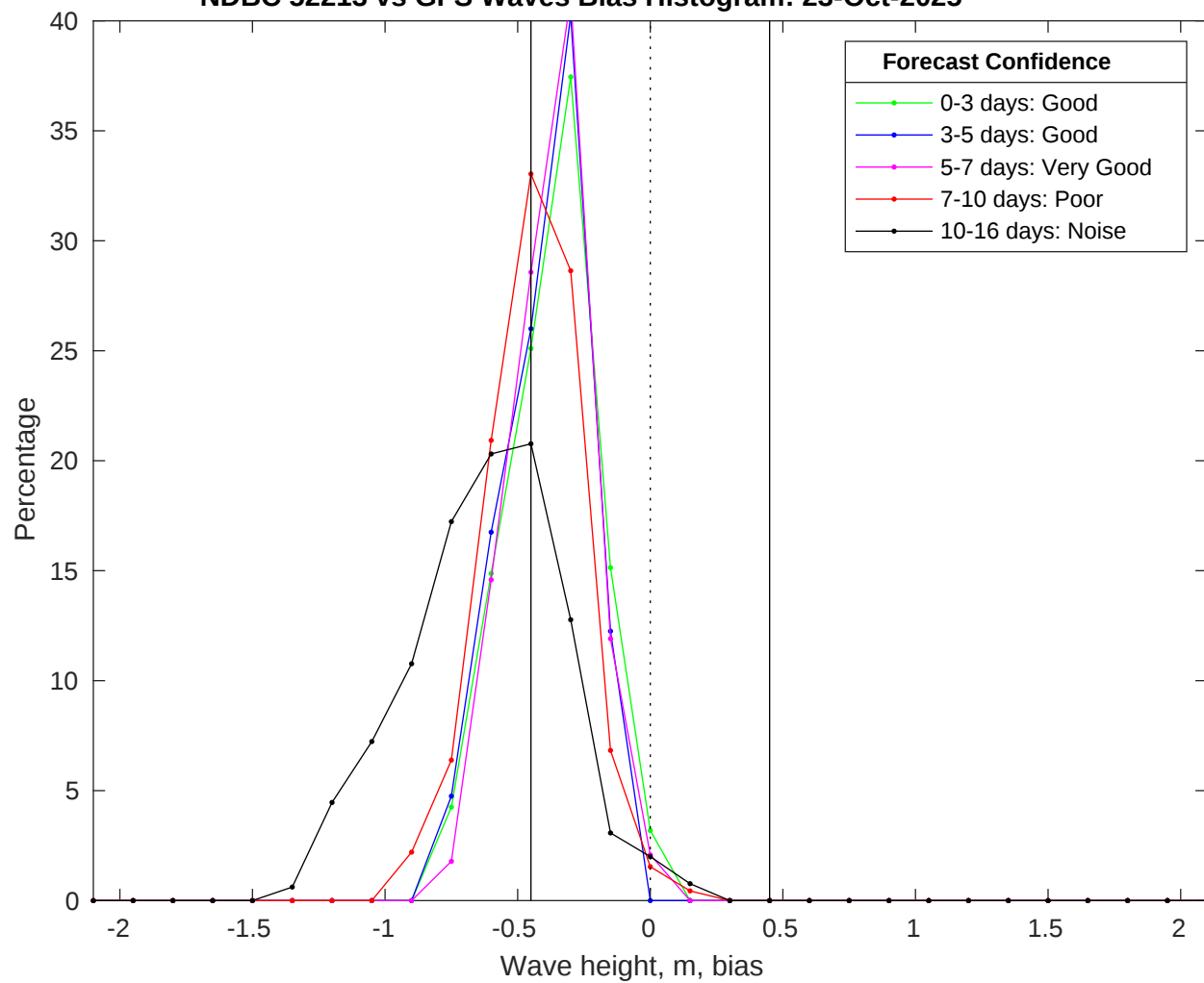
NDBC 52213 vs GFS Waves Bias Histogram: 23-Oct-2025
