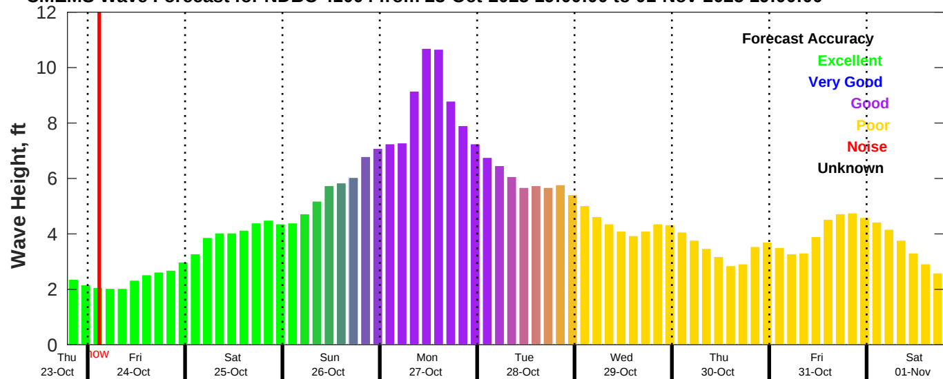
CMEMS Wave Forecast for NDBC 41004 from 23-Oct-2025 19:00:00 to 01-Nov-2025 19:00:00
