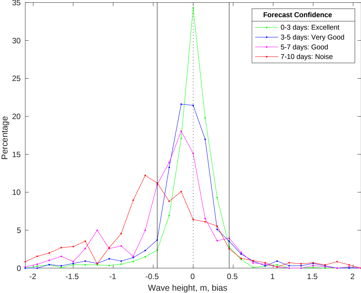
NDBC 41013 vs CMEMS Waves Bias Histogram: 24-Oct-2025
