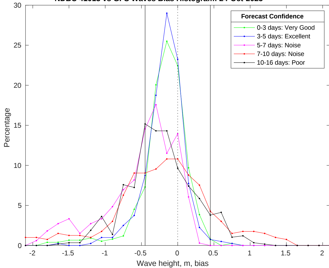
NDBC 41013 vs GFS Waves Bias Histogram: 24-Oct-2025
