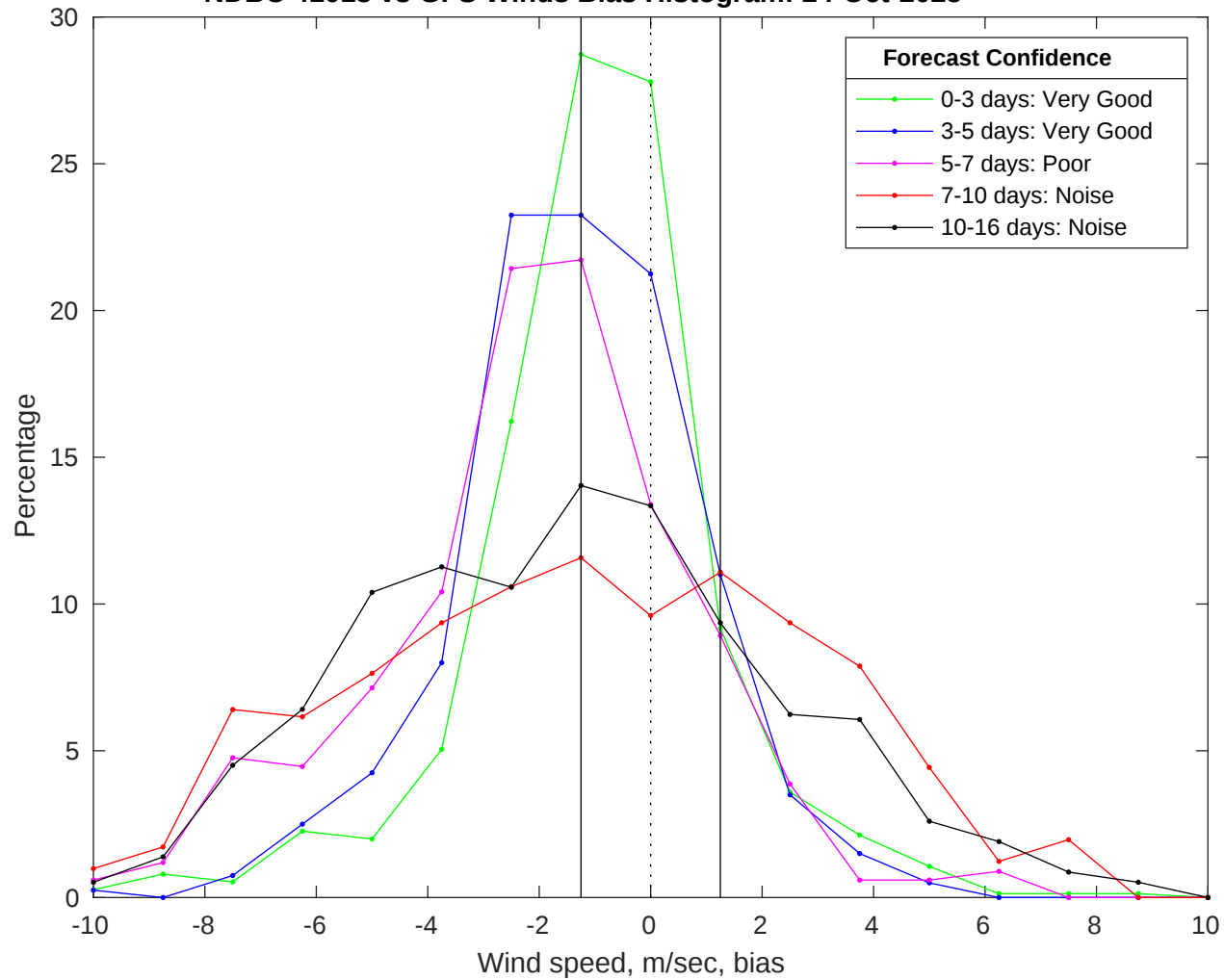
NDBC 41013 vs GFS Winds Bias Histogram: 24-Oct-2025
