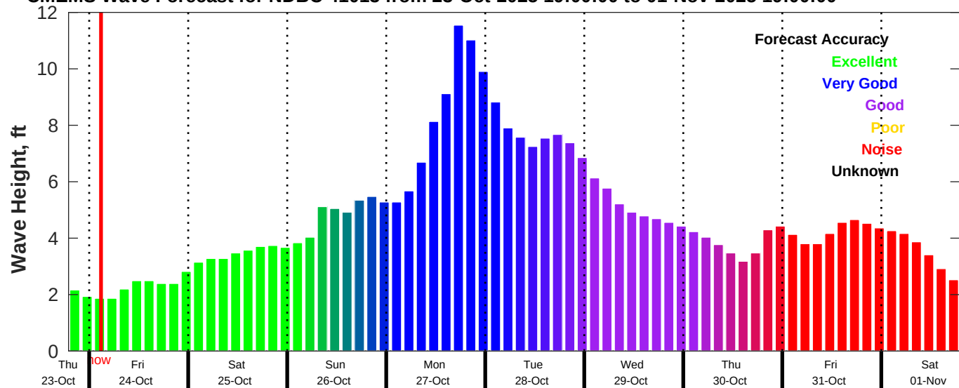
CMEMS Wave Forecast for NDBC 41013 from 23-Oct-2025 19:00:00 to 01-Nov-2025 19:00:00
