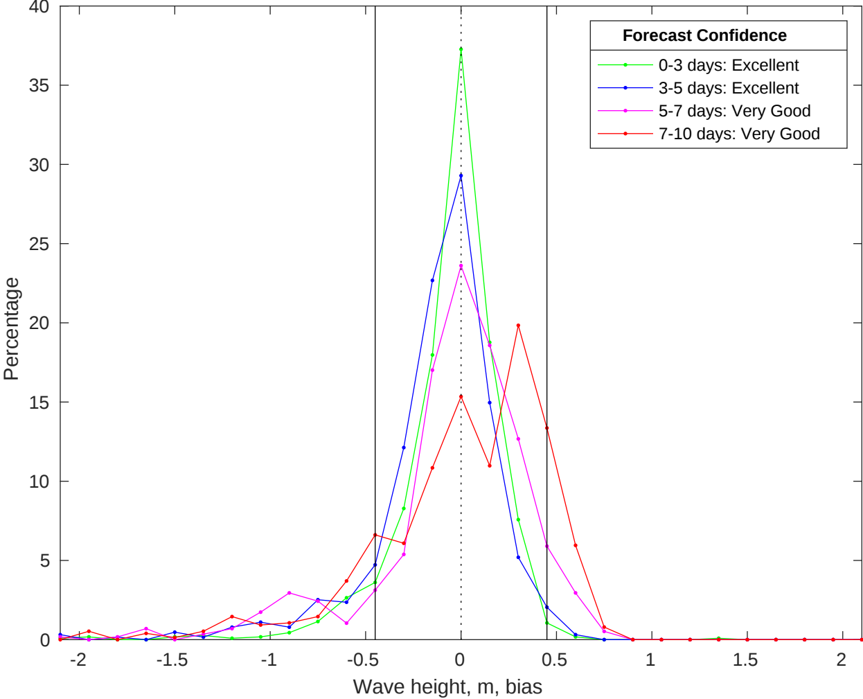
NDBC 41040 vs CMEMS Waves Bias Histogram: 24-Oct-2025
