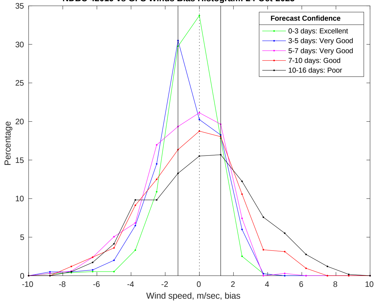
NDBC 42019 vs GFS Winds Bias Histogram: 24-Oct-2025
