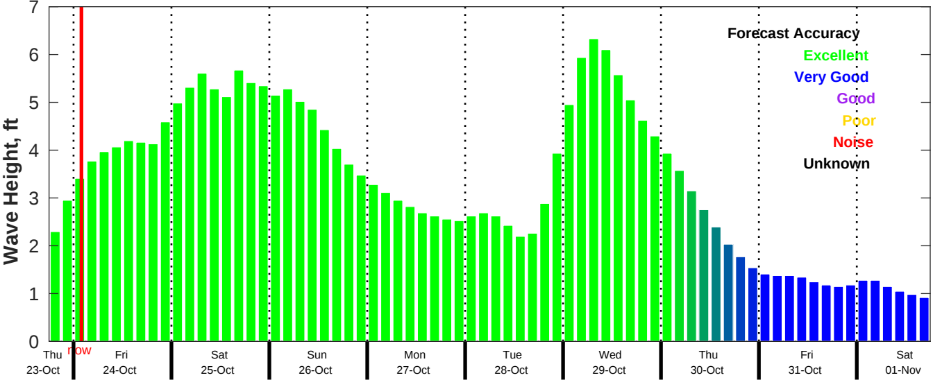
CMEMS Wave Forecast for NDBC 42019 from 23-Oct-2025 18:00:00 to 01-Nov-2025 18:00:00
