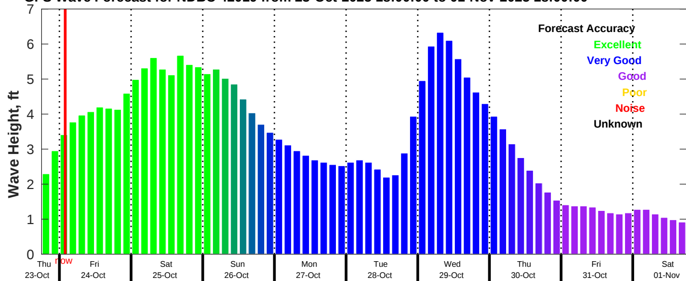
GFS Wave Forecast for NDBC 42019 from 23-Oct-2025 18:00:00 to 01-Nov-2025 18:00:00
