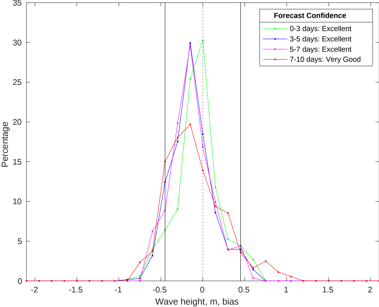
NDBC 42020 vs CMEMS Waves Bias Histogram: 23-Oct-2025
