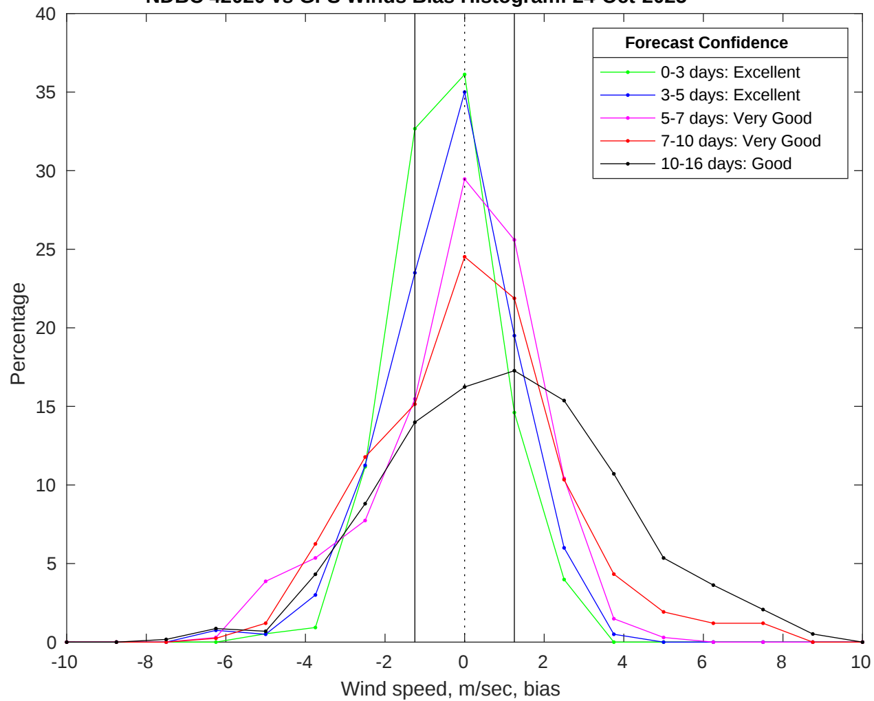
NDBC 42020 vs GFS Winds Bias Histogram: 24-Oct-2025
