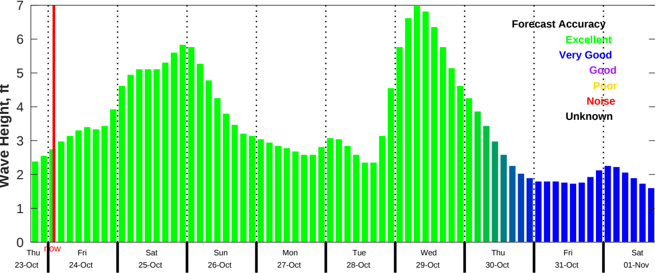
CMEMS Wave Forecast for NDBC 42020 from 23-Oct-2025 18:00:00 to 01-Nov-2025 18:00:00
