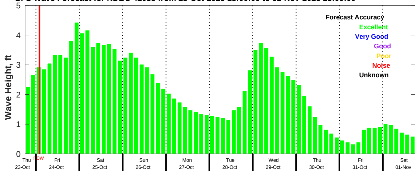
GFS Wave Forecast for NDBC 42035 from 23-Oct-2025 18:00:00 to 01-Nov-2025 18:00:00
