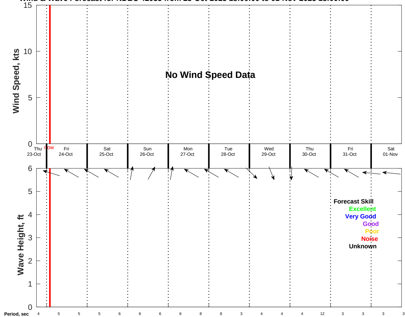
Wind & Wave Forecast for NDBC 42035 from 23-Oct-2025 18:00:00 to 01-Nov-2025 18:00:00
