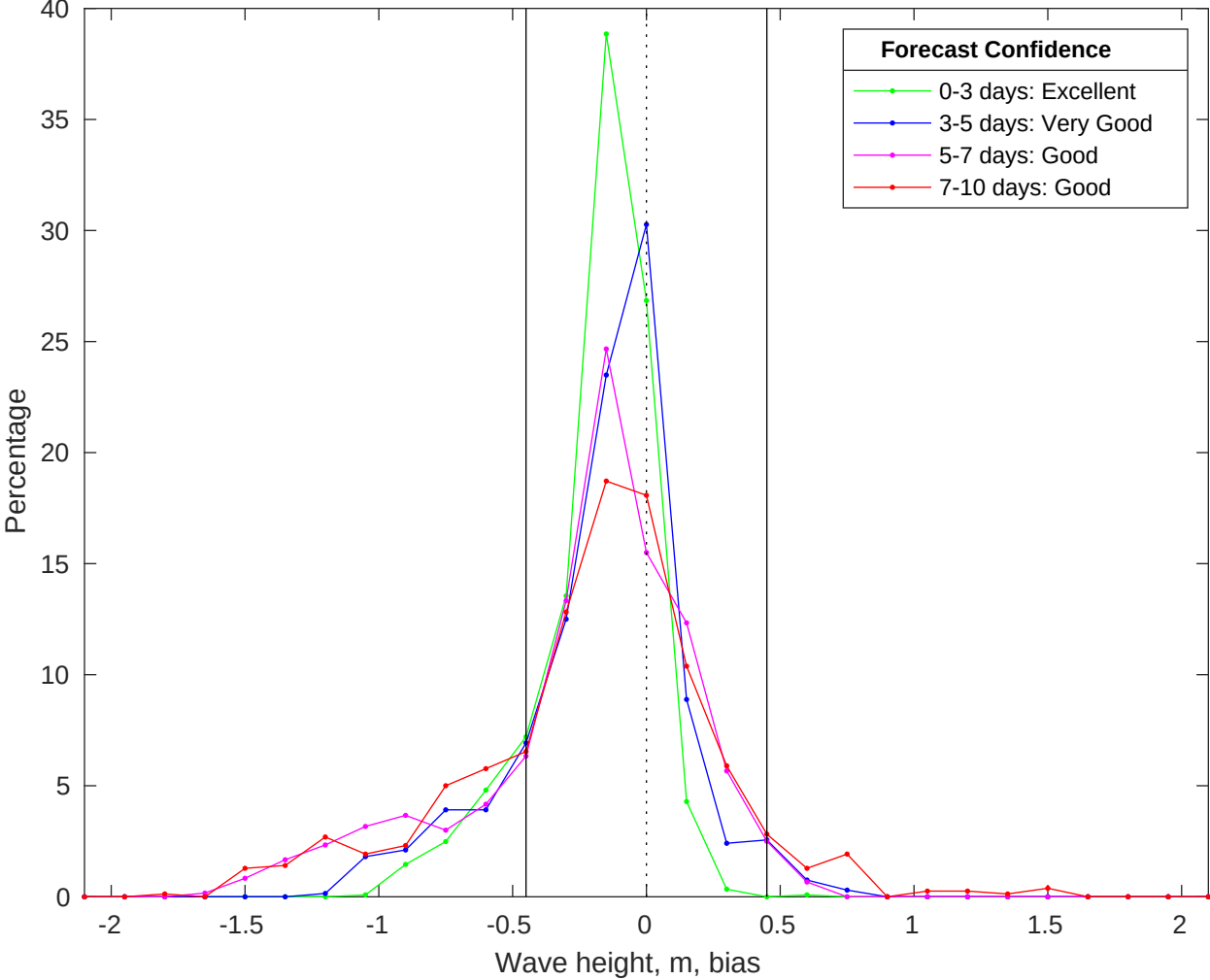
NDBC 42036 vs CMEMS Waves Bias Histogram: 24-Oct-2025
