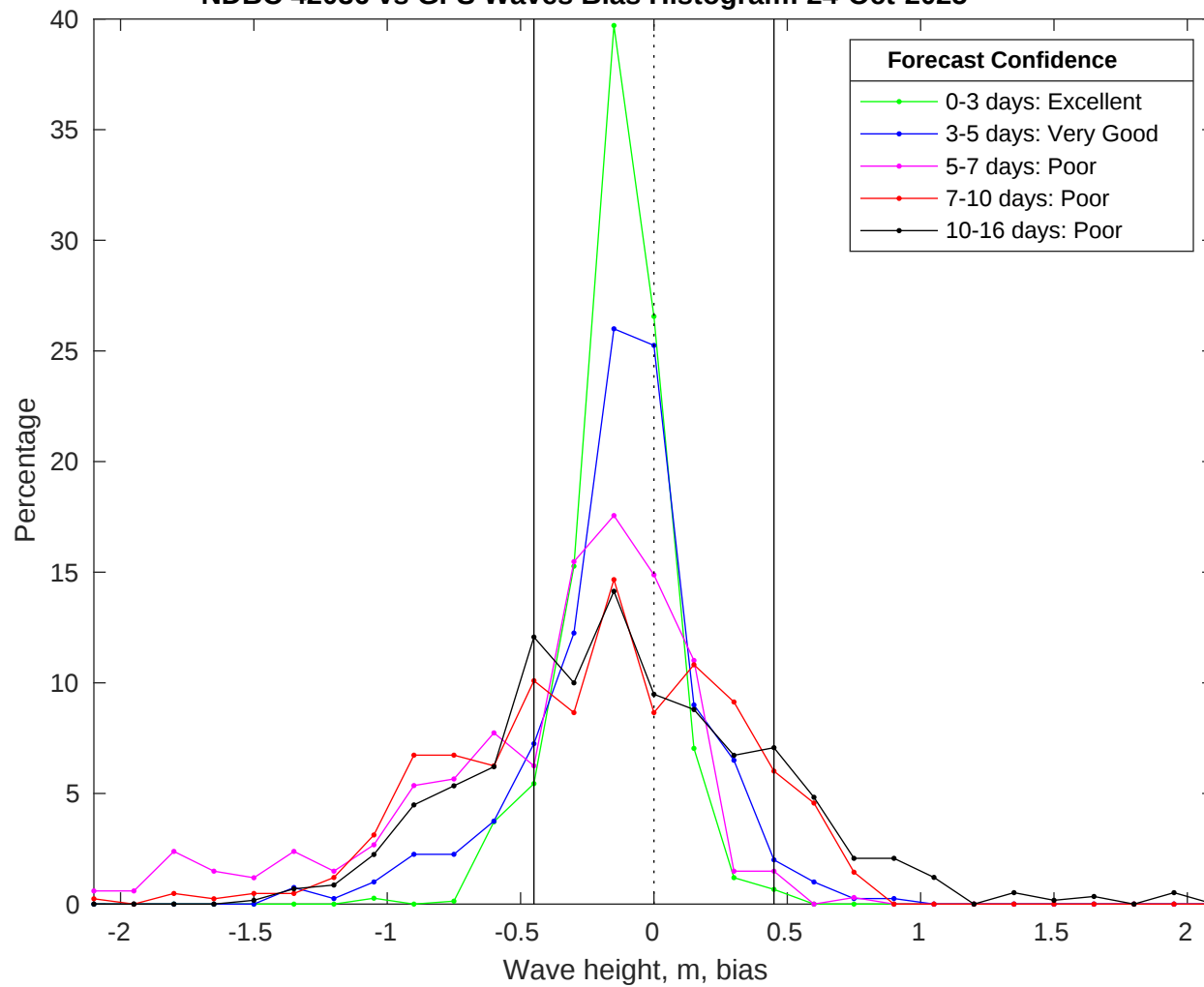
NDBC 42036 vs GFS Waves Bias Histogram: 24-Oct-2025
