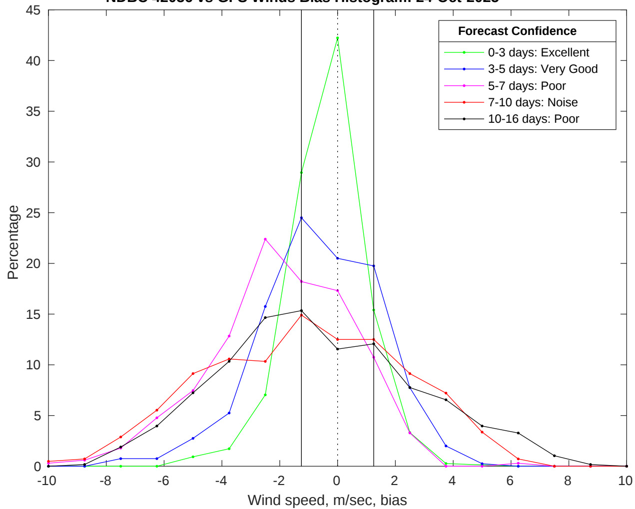
NDBC 42036 vs GFS Winds Bias Histogram: 24-Oct-2025
