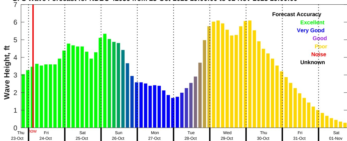
GFS Wave Forecast for NDBC 42036 from 23-Oct-2025 19:00:00 to 01-Nov-2025 19:00:00
