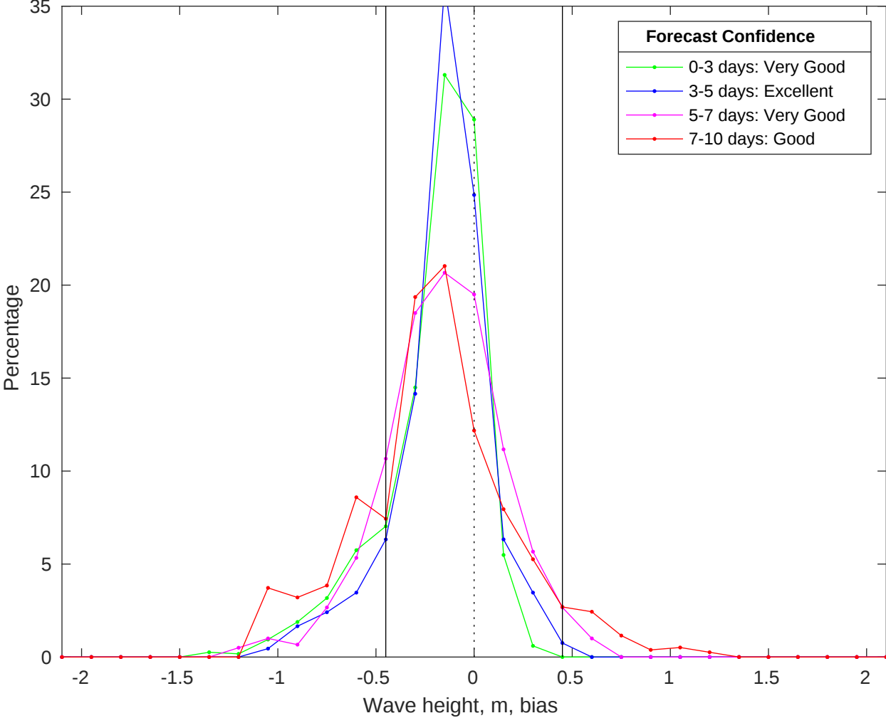
NDBC 42040 vs CMEMS Waves Bias Histogram: 24-Oct-2025
