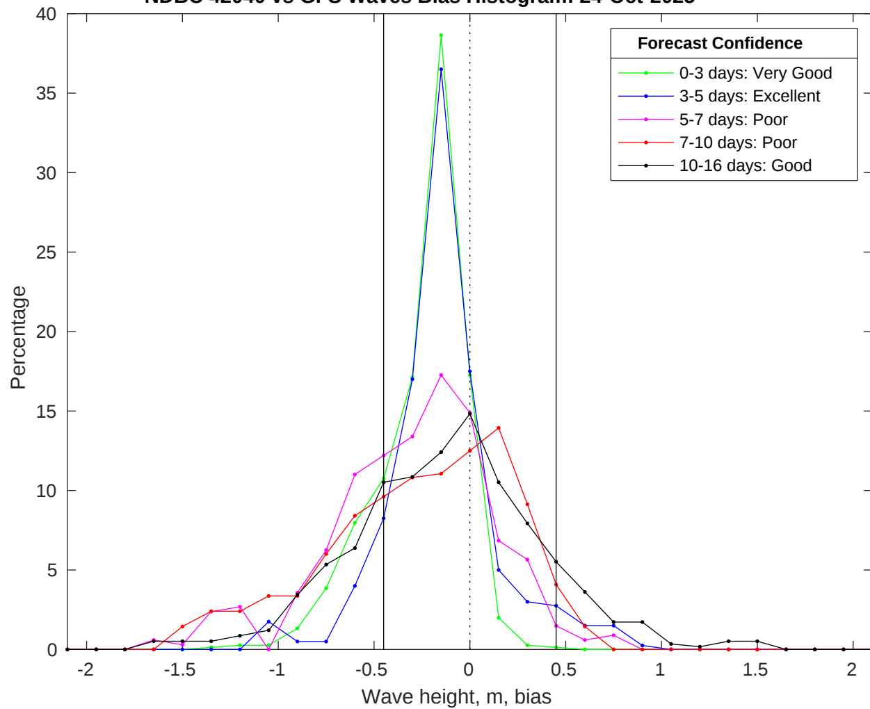
NDBC 42040 vs GFS Waves Bias Histogram: 24-Oct-2025
