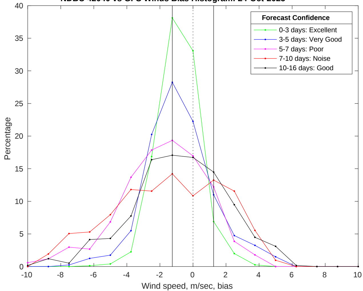
NDBC 42040 vs GFS Winds Bias Histogram: 24-Oct-2025
