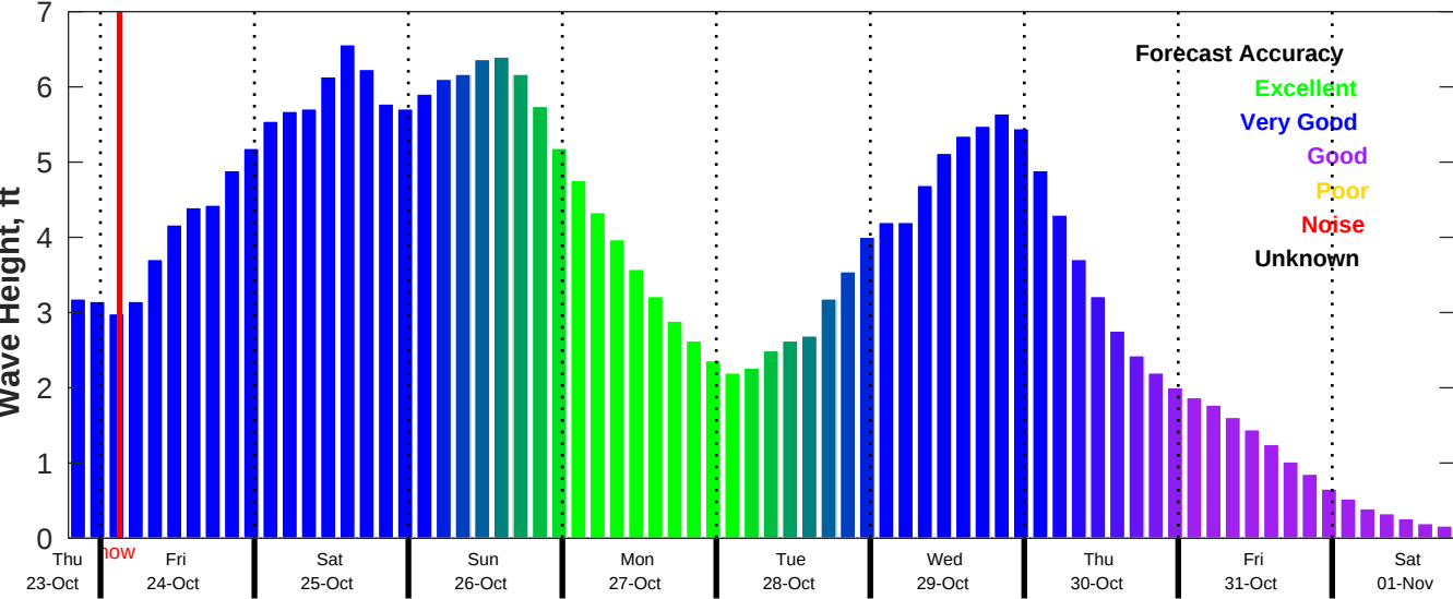
CMEMS Wave Forecast for NDBC 42040 from 23-Oct-2025 19:00:00 to 01-Nov-2025 19:00:00
