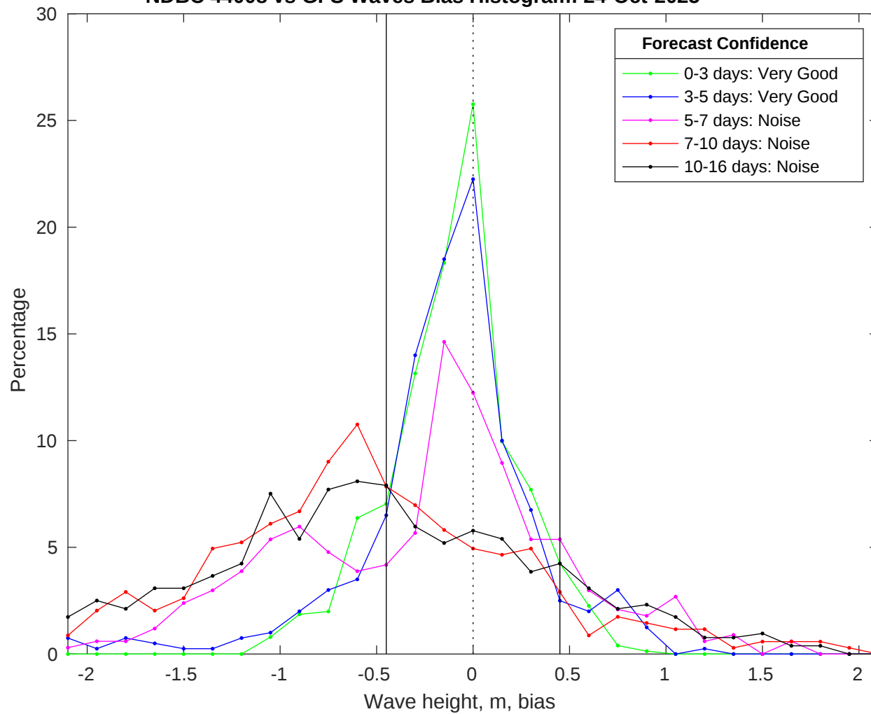
NDBC 44008 vs GFS Waves Bias Histogram: 24-Oct-2025
