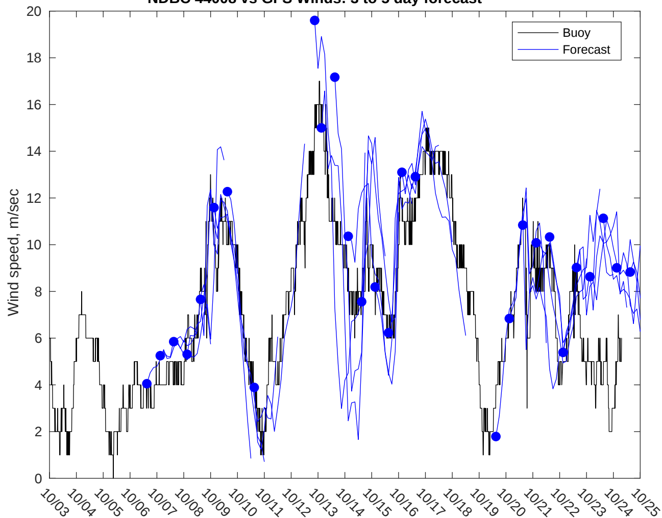
NDBC 44008 vs GFS Winds: 3 to 5 day forecast
