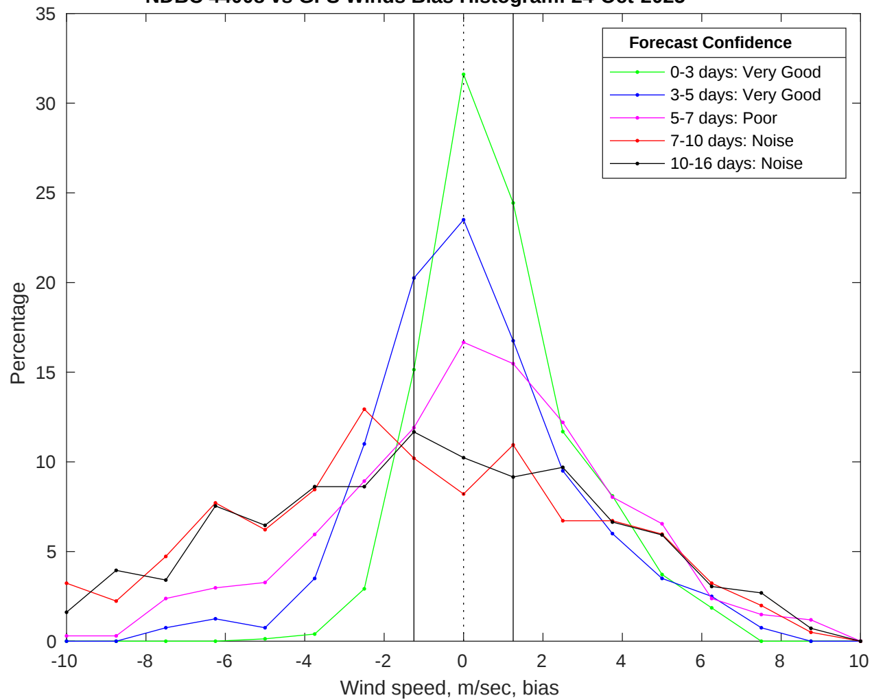
NDBC 44008 vs GFS Winds Bias Histogram: 24-Oct-2025
