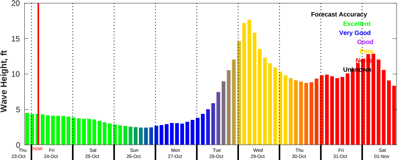
CMEMS Wave Forecast for NDBC 44008 from 23-Oct-2025 20:00:00 to 01-Nov-2025 20:00:00
