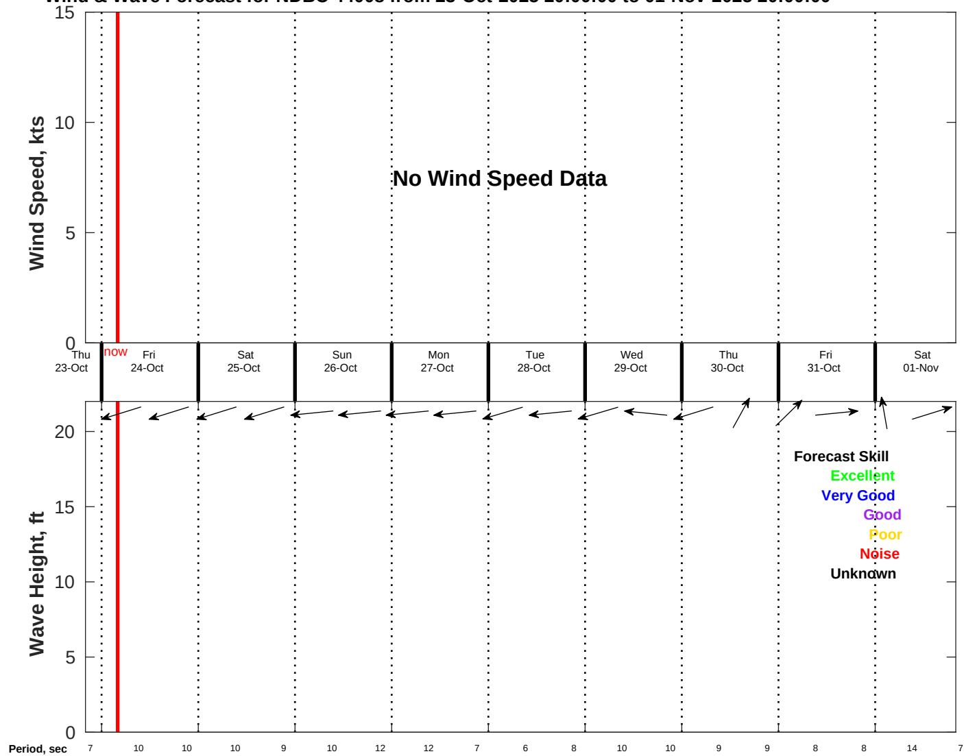
Wind & Wave Forecast for NDBC 44008 from 23-Oct-2025 20:00:00 to 01-Nov-2025 20:00:00
