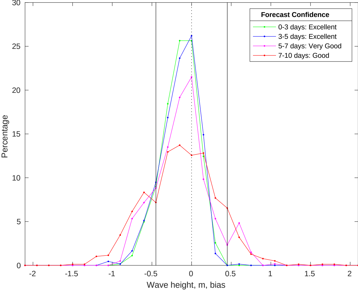
NDBC 46011 vs CMEMS Waves Bias Histogram: 24-Oct-2025
