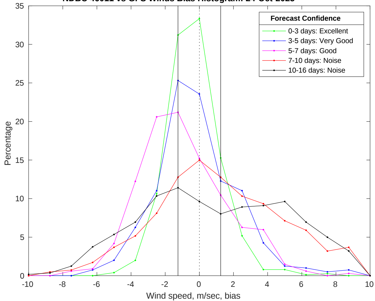
NDBC 46011 vs GFS Winds Bias Histogram: 24-Oct-2025
