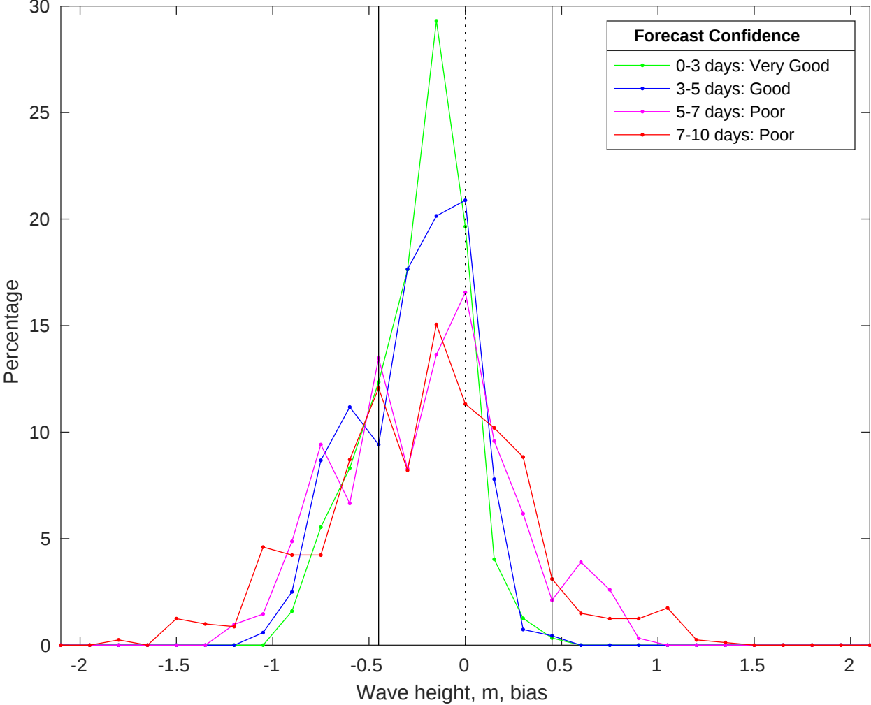
NDBC 46028 vs CMEMS Waves Bias Histogram: 24-Oct-2025
