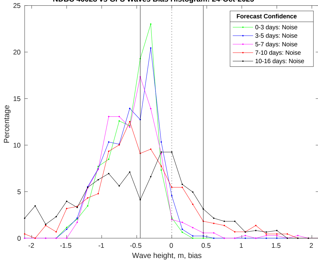
NDBC 46028 vs GFS Waves Bias Histogram: 24-Oct-2025
