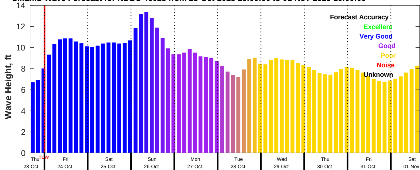
CMEMS Wave Forecast for NDBC 46028 from 23-Oct-2025 16:00:00 to 01-Nov-2025 16:00:00
