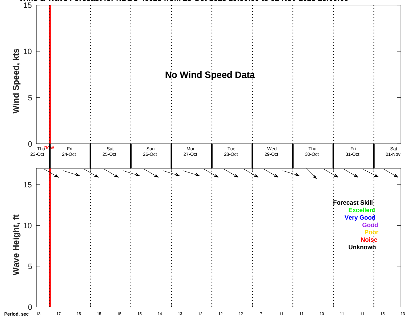
Wind & Wave Forecast for NDBC 46028 from 23-Oct-2025 16:00:00 to 01-Nov-2025 16:00:00
