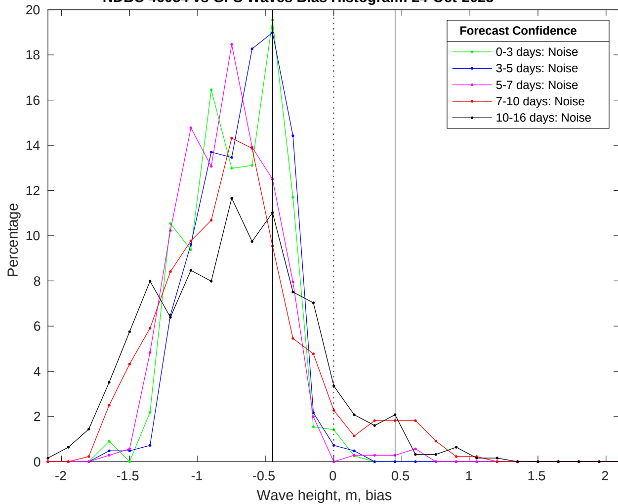
NDBC 46054 vs GFS Waves Bias Histogram: 24-Oct-2025
