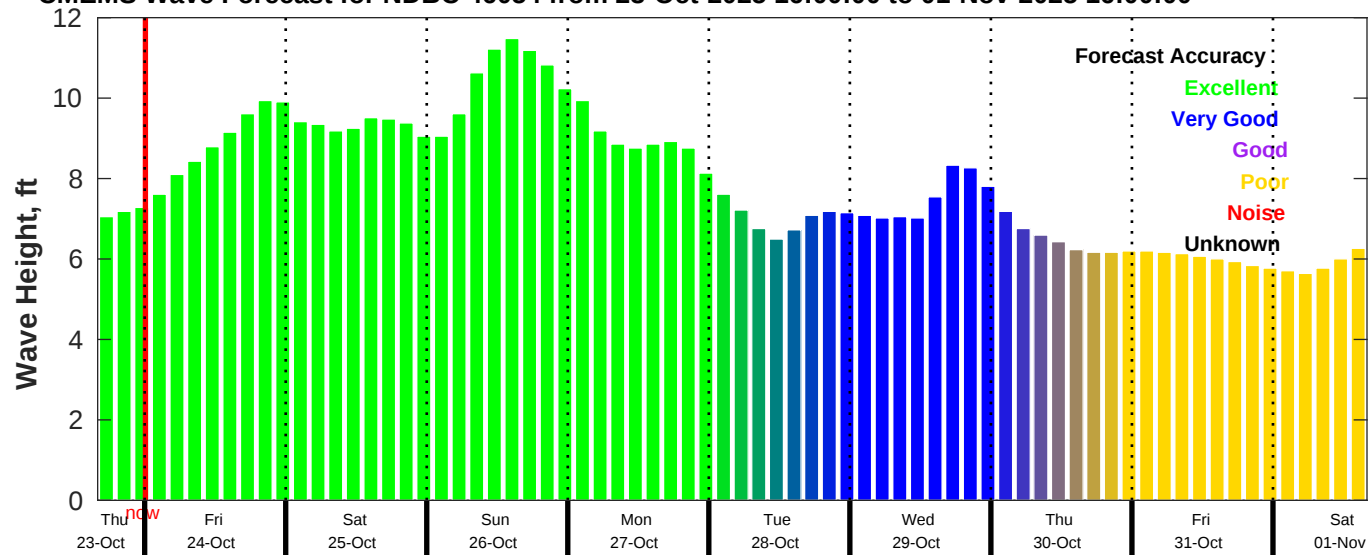
CMEMS Wave Forecast for NDBC 46054 from 23-Oct-2025 16:00:00 to 01-Nov-2025 16:00:00
