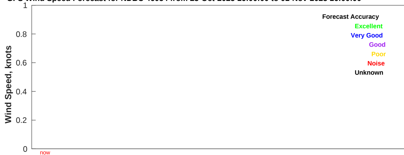
GFS Wind Speed Forecast for NDBC 46054 from 23-Oct-2025 16:00:00 to 01-Nov-2025 16:00:00
