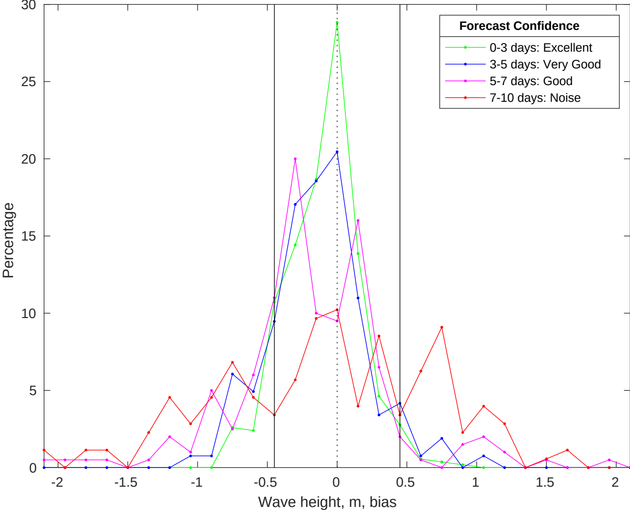
NDBC 46059 vs CMEMS Waves Bias Histogram: 24-Oct-2025
