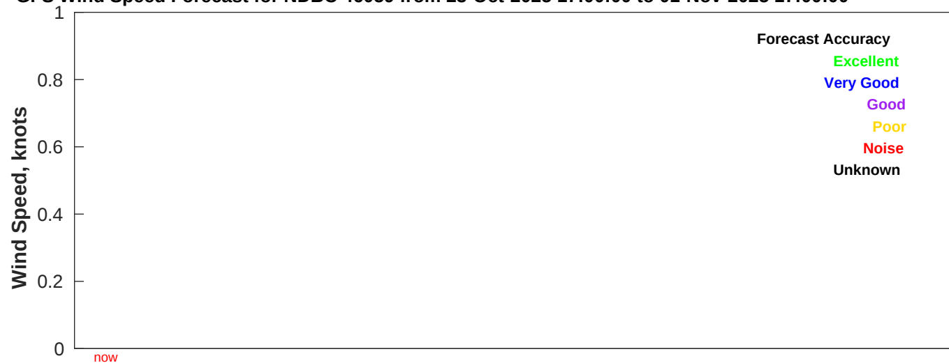
GFS Wind Speed Forecast for NDBC 46059 from 23-Oct-2025 17:00:00 to 01-Nov-2025 17:00:00
