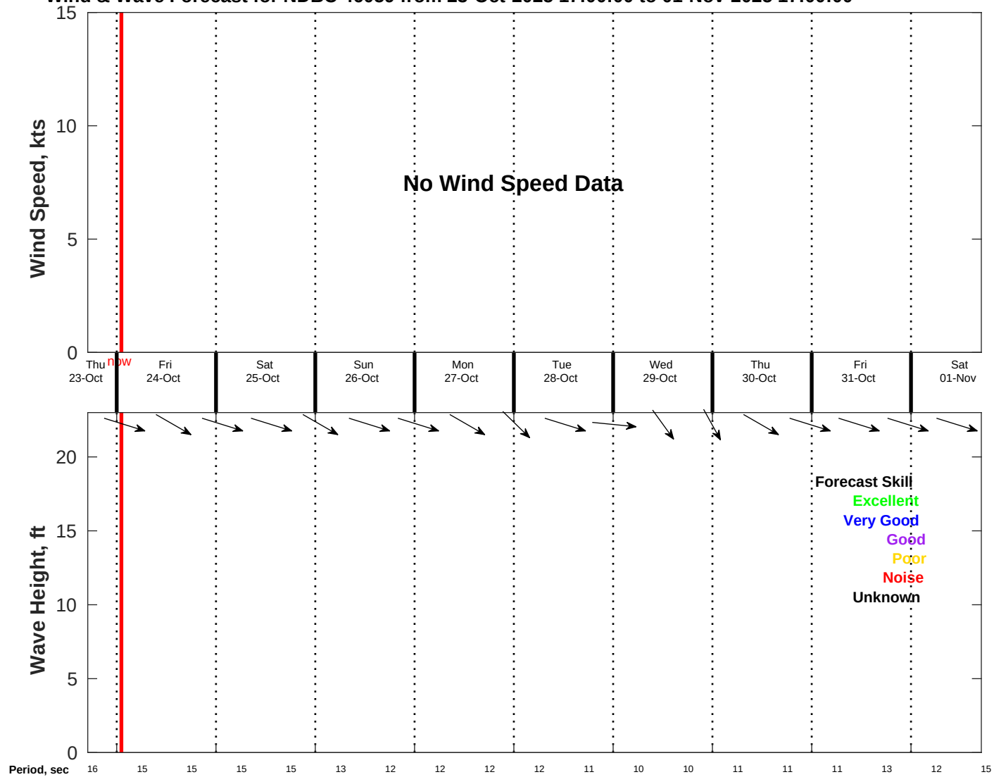
Wind & Wave Forecast for NDBC 46059 from 23-Oct-2025 17:00:00 to 01-Nov-2025 17:00:00
