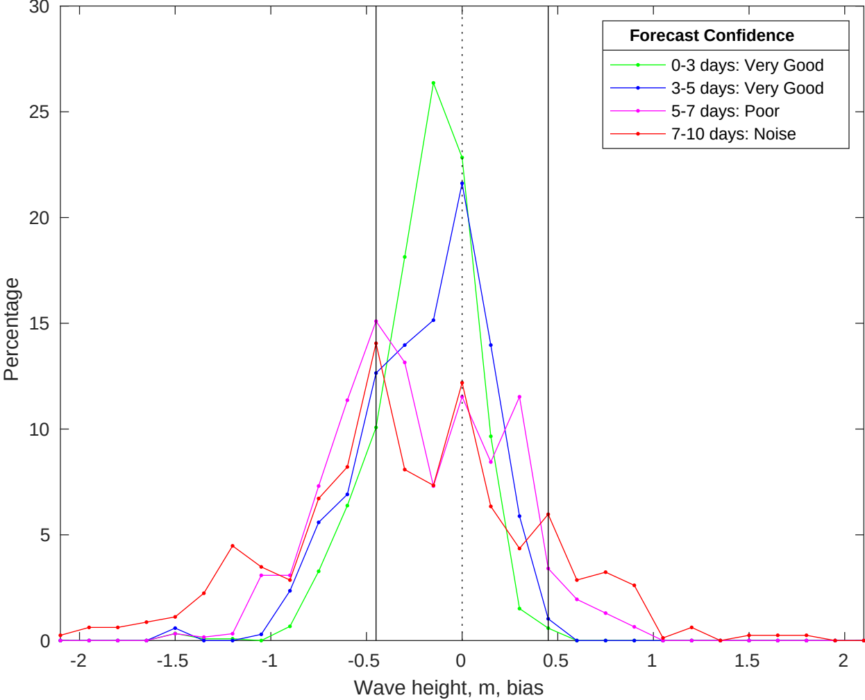
NDBC 46069 vs CMEMS Waves Bias Histogram: 24-Oct-2025
