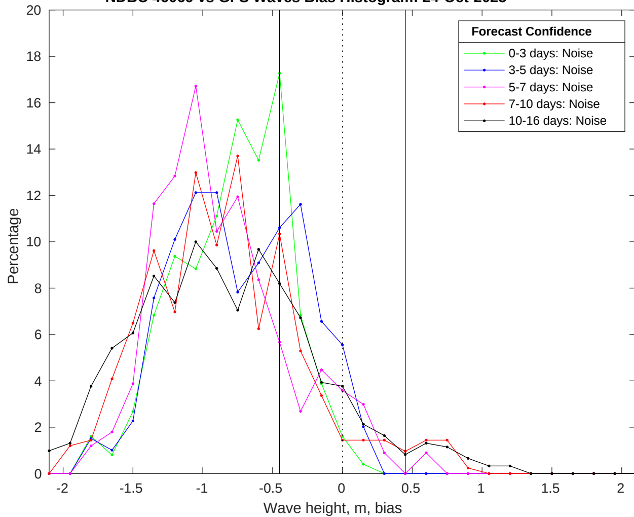
NDBC 46069 vs GFS Waves Bias Histogram: 24-Oct-2025
