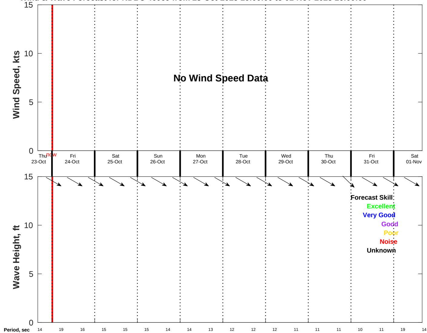
Wind & Wave Forecast for NDBC 46069 from 23-Oct-2025 16:00:00 to 01-Nov-2025 16:00:00
